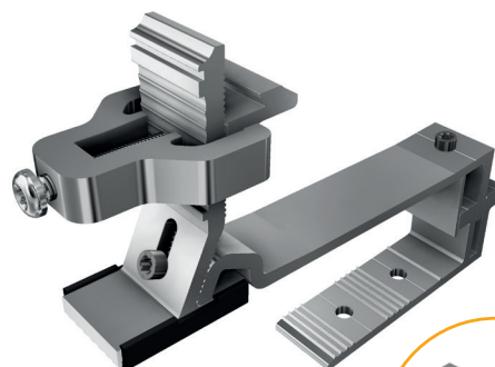
SL Alu Multi Hook Cod. art. 11100-05
